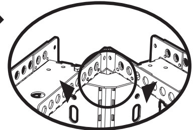
Place NXF35A Array Link Adapters between NXF35U brackets – top adapter shown –
