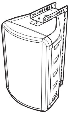
The NX Enclosure can easily be mounted after the NFX35U bracket has been installed
