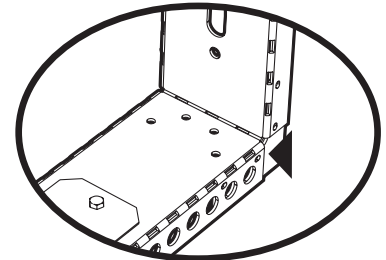
Mounting hole location on the NXF35U bracket
