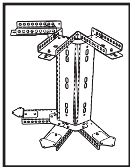
The NXF350U Bracket with the optional NXF350A Installed. Three enclosure array.
