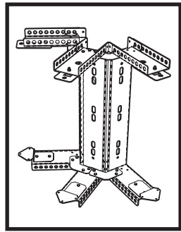
The NXF35U Bracket with the optional NXF35A Installed. Three enclosure array.
